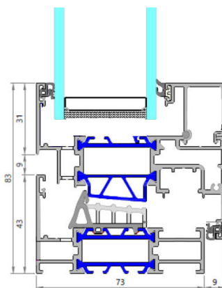
Doorsnede "Flat" (*)
